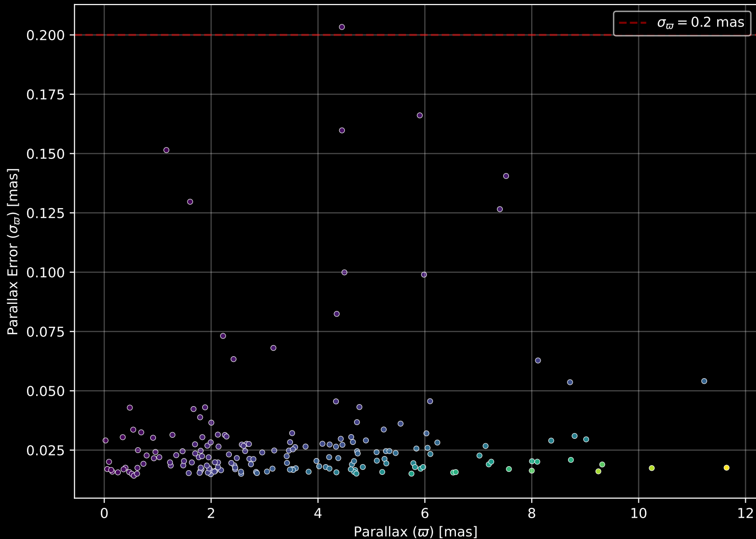
APOGEE DR17 Field: [048+88_MGA] Parallax Quality (n= 182)
