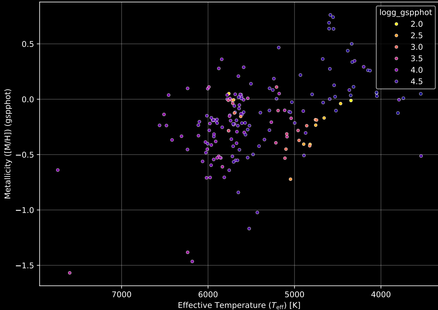
APOGEE DR17 Field: [048+88_MGA] Stellar Population Parameters (n= 182)
