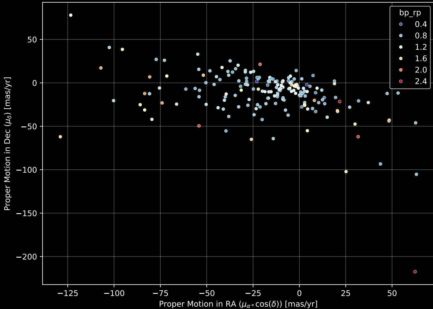
APOGEE DR17 Field: [048+88_MGA] Proper Motion Diagram (n= 182)
