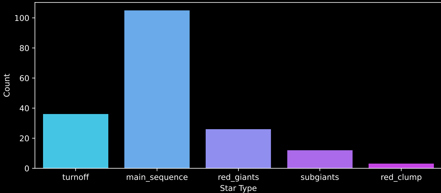
APOGEE DR17 Field: [048+88_MGA] Count plot of Star Type
