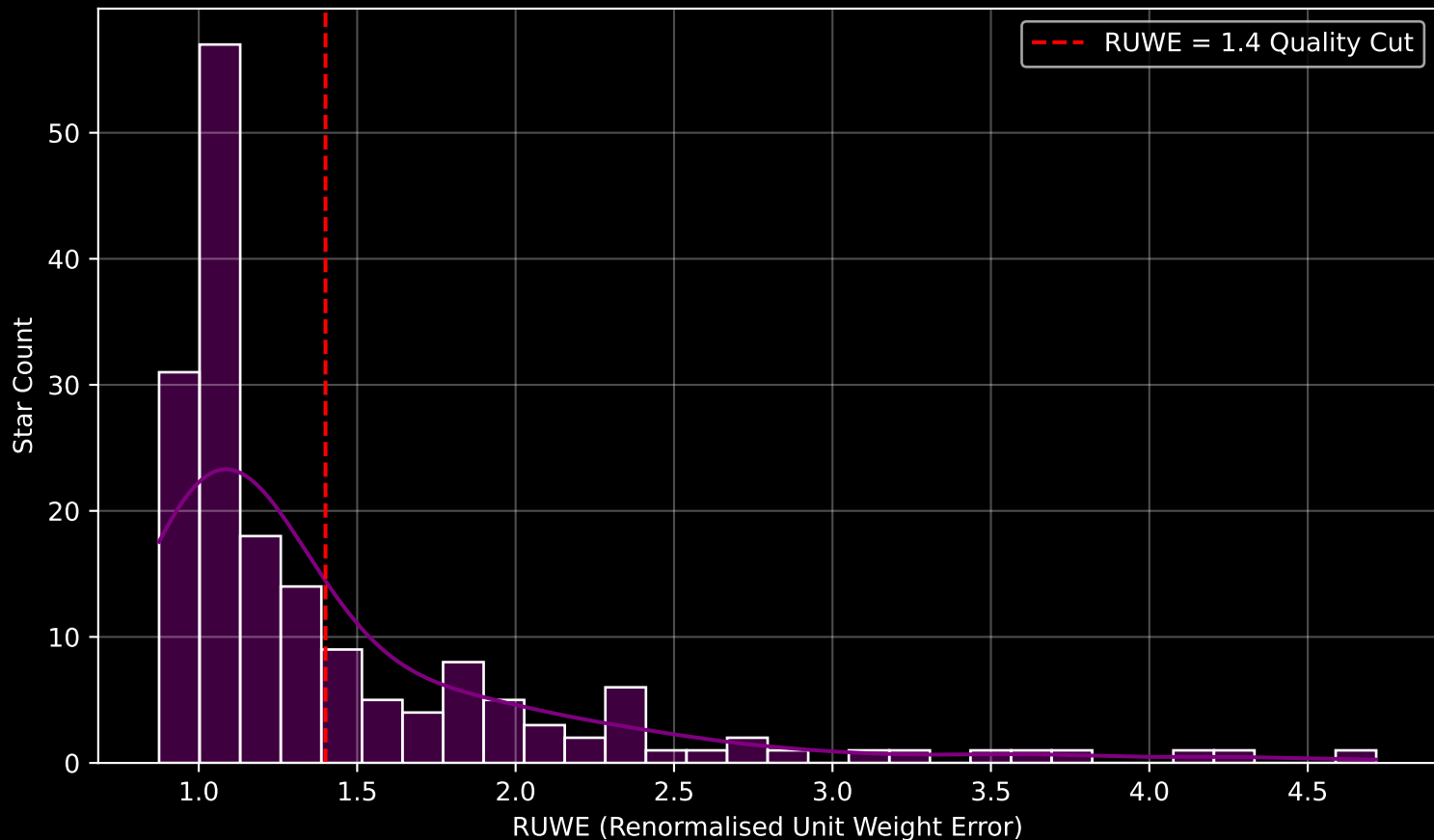
GAPOGEE DR17 Field [048+88_MGA] RUWE Distribution (n= 175)
